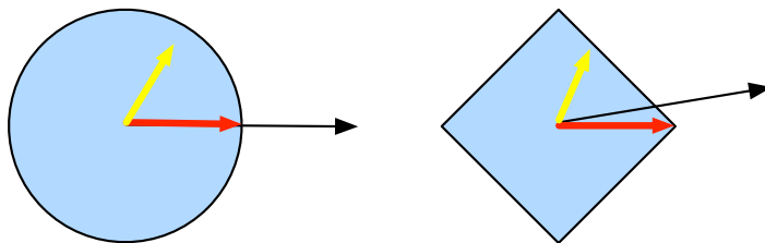
图11.2.4: Convex Projections.
