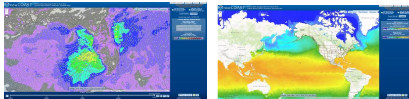
Global SST analysis updated once/day
