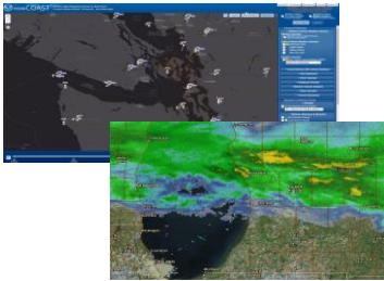
Wx radar images updated every 4 mins
