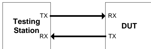
Figure 4 - 115 Test Setup for 1000BASE-T Devices
