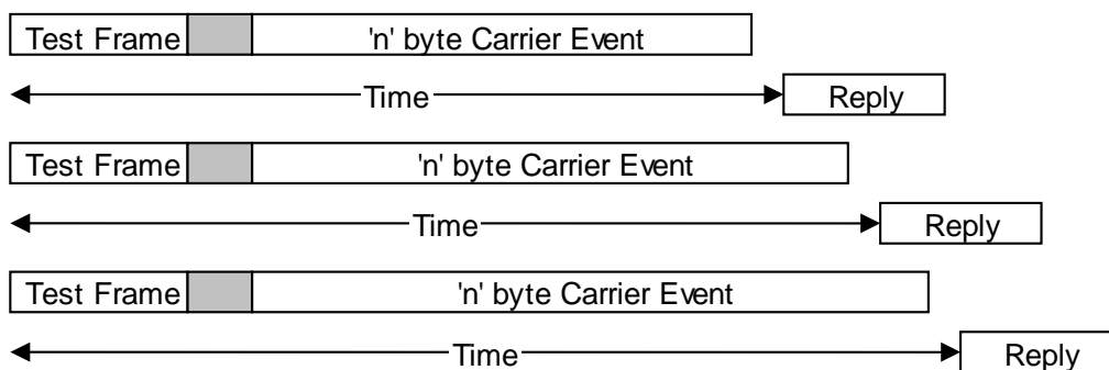
Figure 4 - 44 Defer to carrier sense while frame waiting
