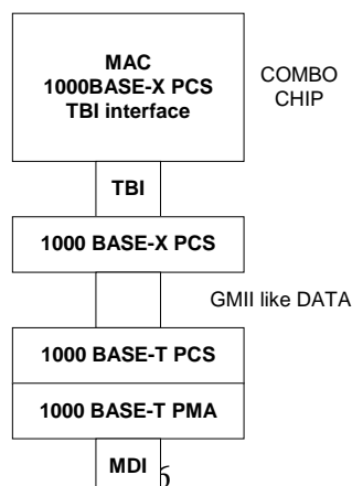
Figure 4 - 5 1000BASE-T PHY Utilizing a MAC/1000BASE-X PCS Combo Chip
