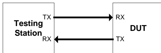
Figure 4 - 21 Test Setup#1 for 100BASE-X Devices
