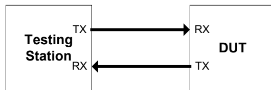
Figure 4 - 24 Test Setup #2 for 1000BASE-X Devices
