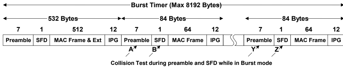
Figure 4 - 11 Collisions during preamble and SFD outside of slotTime (Burst Mode)
