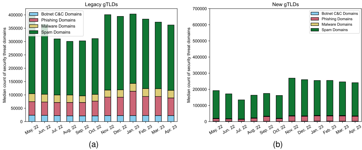
Figure 2: Breakdown of domains identified as security threats across all DAAR threat types over time
