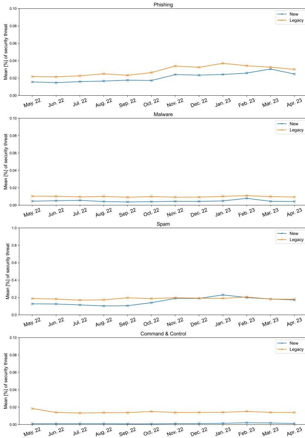
Figure 8: Average percentage of security threat in TLDs across different threat types over time
