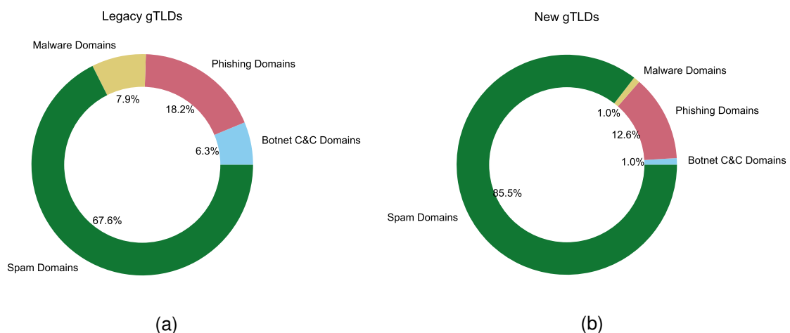
Figure 1: Breakdown of domains identified as security threats across all DAAR threat types
