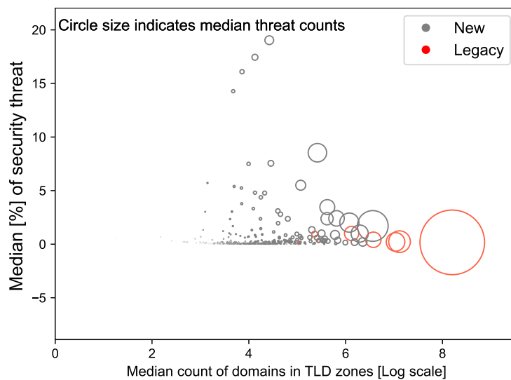
Figure 5: Percentage of domain names identified as security threats vs. median count of domains in TLD zones
