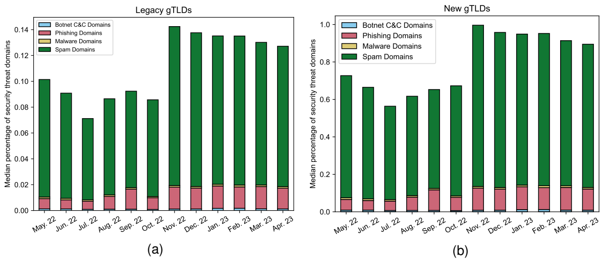
Figure 3: Breakdown of percentage of domains identified as security threats in proportion to all domains in zone files across all DAAR threat types over time [note:y-axis scales differ across graphs]
