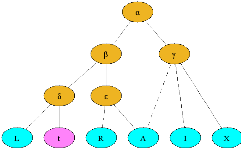
Figure 34: Example stemma
