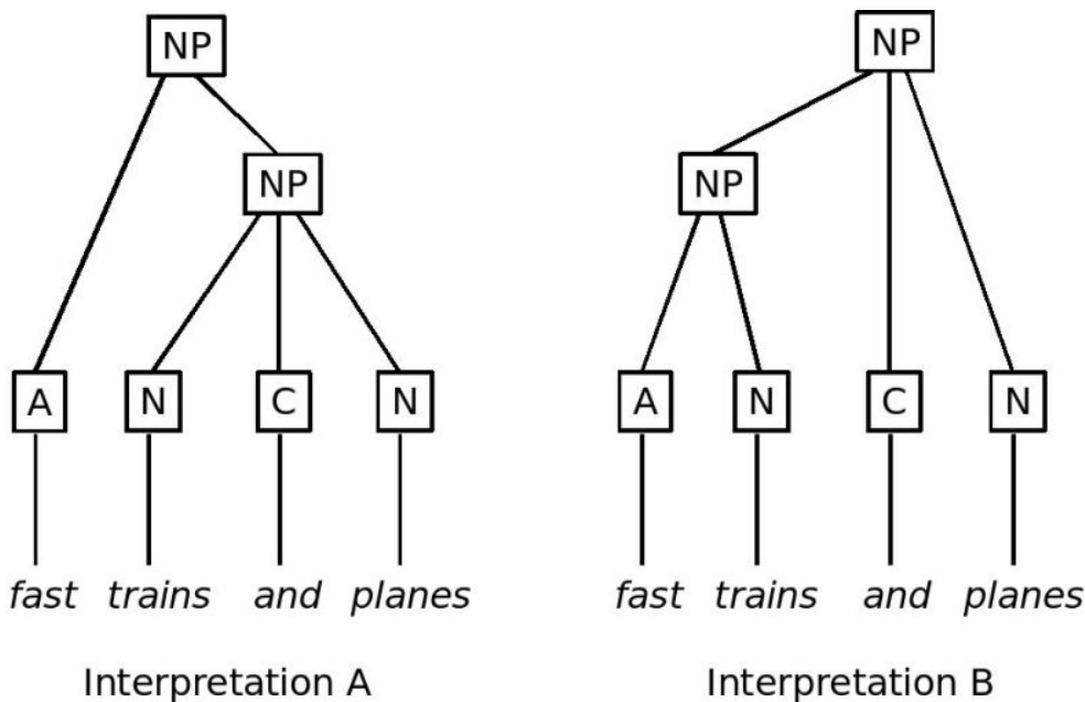
Figure 35: Two interpretations of the phrase Fast trains and planes
