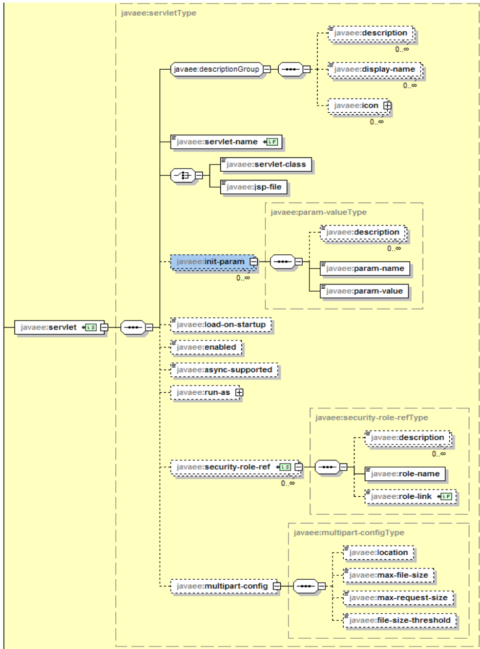
FIGURE 14-5 servlet Element Structure
