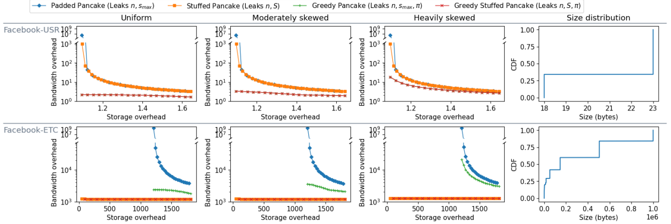
Figure 13: Bandwidth vs. storage overhead across schemes with different leakage (continued from §1.1). We use real-world workloads Facebook-USR (top) and Facebook-ETC (bottom) from Facebook Memcached deployments [4], and Zipf access patterns with varying skew (left to right). The rightmost column shows the dataset’s object size CDF. Bandwidth overheads for schemes that do not leak object sizes start from the minimum storage footprint required for security, i.e., n \cdot s_{max} . The y-axes are in log-scale broken between bandwidth overheads 1200\text{--}2e5 \times (Facebook-USR) and 70000\text{--}2e5 \times (Facebook-ETC).
