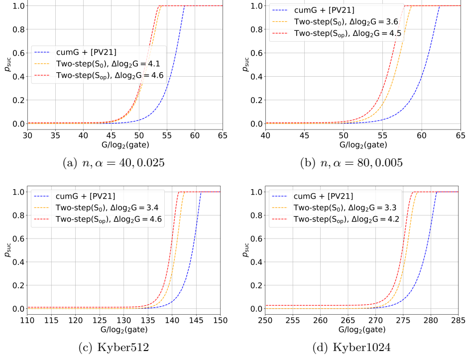
Fig. 3. The relation among the growth of cumulated cost and the success probability. Comparison between the output of cumulated Cost Version of [21] (Algorithm 1) and Two-step mode (Algorithm 2, this work) for lwe challenge (n, \alpha) \in \{(40, 0.025), (80, 0.005)\} and on Kyber 512 and Kyber 1024 [1]. “Two-step( S_0 )” uses a trial progressive BKZ+Pump in Two-step mode to estimate security. “Two-step( S_{\text{op}} )” uses a progressive BKZ+Pump with the optimized strategy selected by EnumBS [28] in Two-step mode to estimate security. We set \Delta \log_2 G as the gate count difference between our estimator and the leaky-LWE-estimator both using the same gate count 6 .
