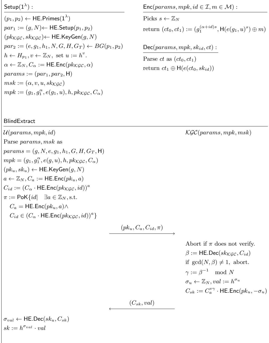
Fig. 1. Oblivious IBE Construction with identity space \mathcal{I} = \mathbb{Z}_N and message space \mathcal{M}
