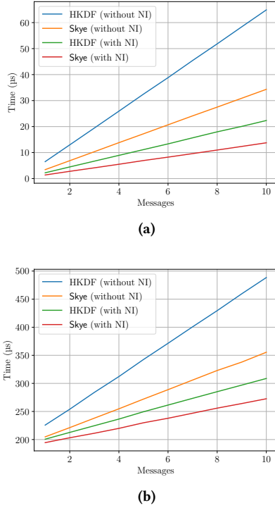
Figure 7: (a) The mean time (in \mu\text{s} ) required to encrypt n messages in the Signal Protocol implementation using Skye and HKDF. (b) The mean time (in \mu\text{s} ) required to encrypt (on sender side) then decrypt (on receiver side) n messages, and then encrypt (on receiver side) and decrypt (on sender side) another n messages in the Signal Protocol implementation using Skye and HKDF. In both cases, the measurements were performed for variants with and without AES-NI and SHA-NI support. The encrypted messages were of less than 16 characters. All measurements were repeated 10^3 times.
