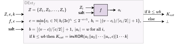
Figure 1: \text{DExt}_f : A (U_Z, b(2\epsilon)^c/2) -extractor (with upto wb bits of extraction) parameterized by a relatively small and weak (U_{Z_i}, \epsilon) -extractor f (with upto w bits of extraction). Here U_{Z_i} and U_Z denote random variables distributed according to the sampling of Z_i s from S_i s for all i s and of corresponding Z from the Cartesian product of all S_i s, respectively.
