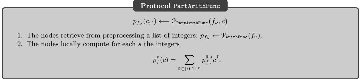
Fig. 6: Protocol to compute the coefficients of the partial application of a Boolean function in two variables
