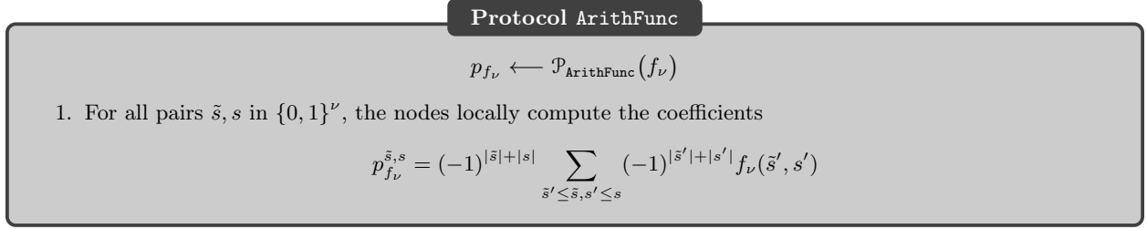
Fig. 5: Protocol to compute the coefficients of a Boolean function in two variables
