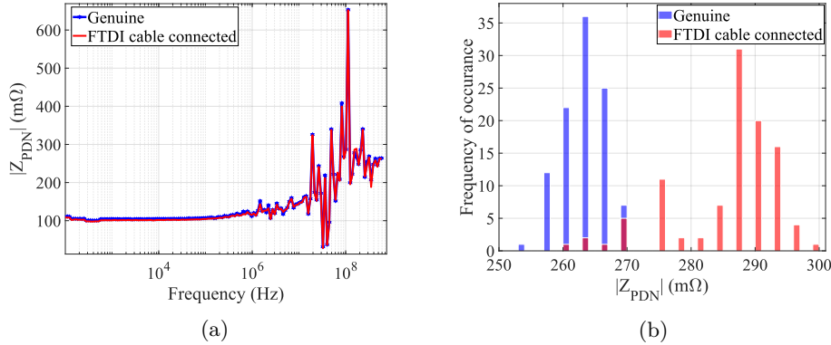
Figure 14: Connecting the FTDI cable to one of the I/O ports. (a) The mean of 105 impedance profile signatures. (b) Histogram representation ( f = 169.85 MHz).
