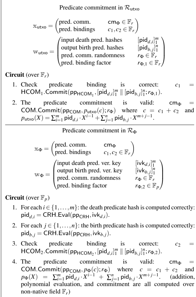
Figure 13: Relation snippet for optimized predicate commitment.
