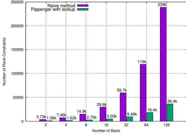
Figure 9: Circuit complexity for variable-based MSM.
