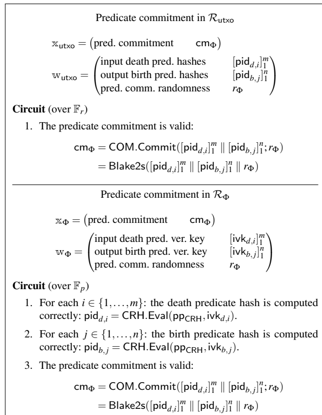
Figure 12: Relation snippet for predicate commitment in [14].
