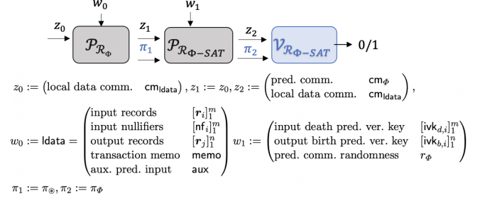
Figure 1: Casting \mathcal{R}_\Phi proving into a two-step IVC (with different step function at each step).
