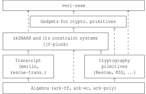
Figure 8: Stack of libraries comprising VERIZEXE.
