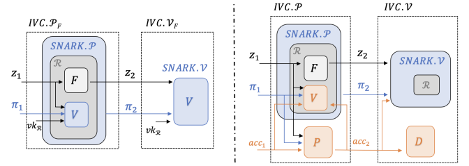
Figure 2: IVC from SNARK compositions (left) v.s. IVC from accumulation schemes (right). Blue boxes are SNARK prover \mathcal{P} and verifier \mathcal{V} for the relation \mathcal{R} , and orange boxes are accumulation prover \mathcal{P} , verifier \mathcal{V} (more lightweight than a SNARK verifier) and decider \mathcal{D} . z_1, z_2, \pi_1, \pi_2 in both schemes are the same as those in Fig. 1 where F is the step function that calculates the predicate commitment cm_\Phi using Pedersen Commitment over the hashes of the predicate verifying keys. There are a few inputs dropped from the diagram for visual clarity, e.g. witness w_1 as an input to the IVC prover in both diagrams; SNARK verifying key vk_{\mathcal{R}} for the SNARK verifier inside the IVC verifier on the right diagram.
