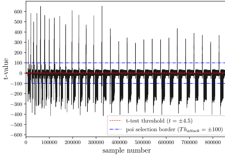
Fig. 4: Resulting t-values used for identifying points of interest using the side-channel described in Section 4.1. The marked Th_{\text{attack}} is used as a threshold for the actual attack.
