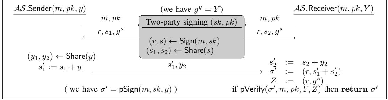
Figure 4: In gray: two-party ECDSA signing provided by [41], [52]. In clear: extension for weak adaptor signing
