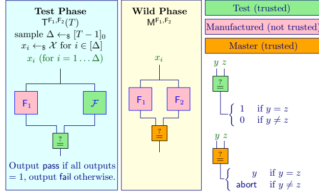
Fig. 2. Construction \Pi_2^* (discussed in Sec. 2.9), which is (c, \frac{c'}{T}) secure for history-independent Trojans.
