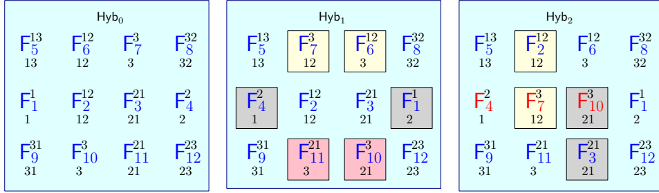
Fig. 7. Hybrids with the circuits and their corresponding plaited hardcoded history and input streams (above and below each circuit in black respectively). In \text{Hyb}_2 , F_4^2 and the plaited circuit F_7^3 F_{10}^3 (in red) are history independent.
