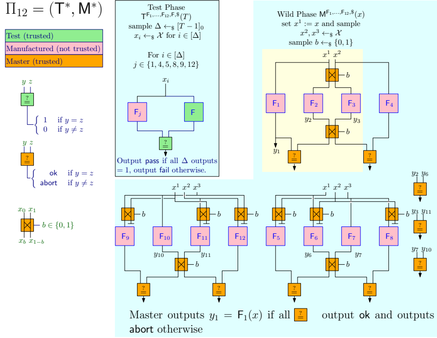
Fig. 3. Construction \Pi_{12} for which we prove optimal Trojan-resilience as stated in Thm. 1. Very informally, the security proof is by contradiction: via a sequence of hybrids an attack against \Pi_{12} is shown to imply an attack where the yellow part basically corresponds to \Pi_2^* with two history independent circuits. This attack contradicts the security of \Pi_2^* as stated in Thm. 2.
