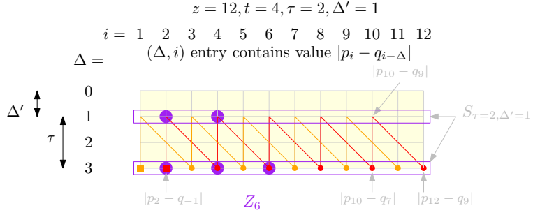
Fig. 5. Illustration of the main variables used in the proof of Lem. 5.
