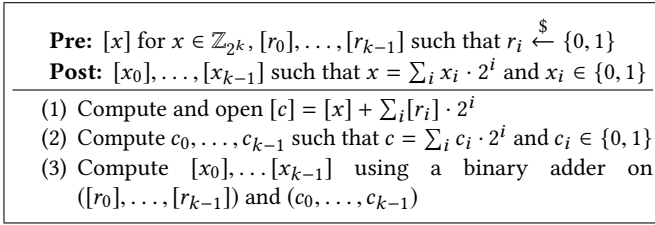
Figure 5: Bit decomposition modulo 2^k using random bits.
