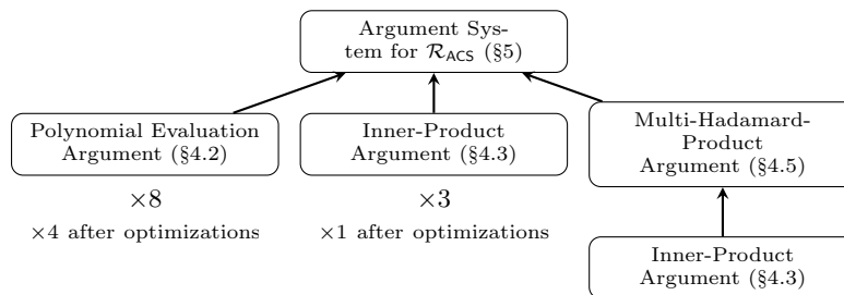
Fig. 1: Overview of the techniques involved to construct our argument system for general computation. We achieve concrete optimizations by batching and instantiating in the Algebraic Group Model [37]. More details are provided in supplementary section F.
