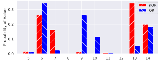
Figure 6: Probability distribution for attack results
