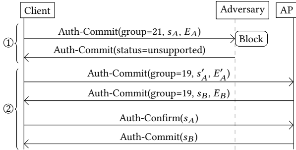
Figure 3: Downgrade attack against SAE’s group selection: a man-on-the-side can force the client (initiator) into using a different cryptographic group during the SAE handshake.
