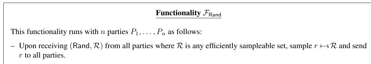
Figure 11: Coin-tossing functionality.
