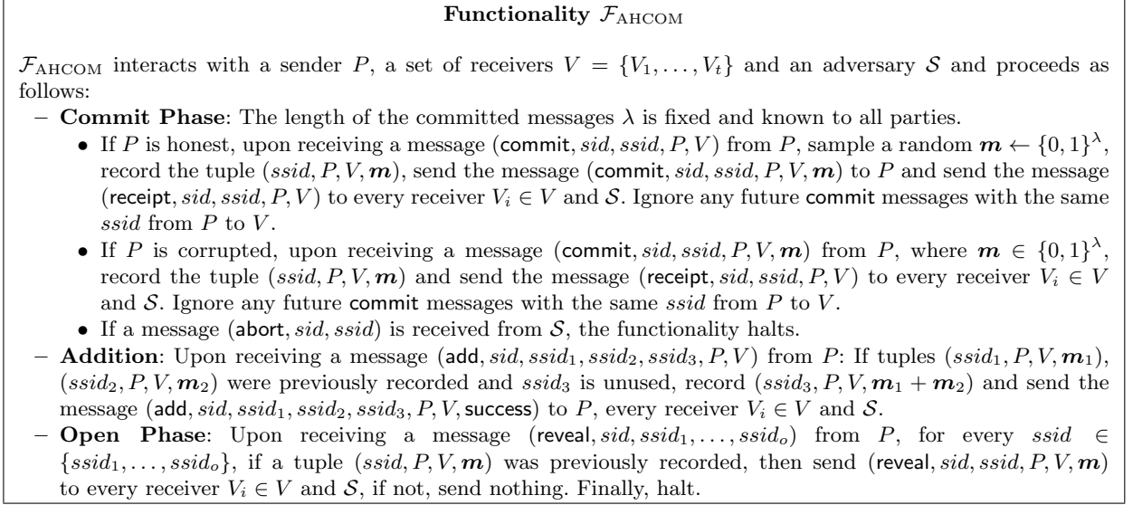
Fig. 2. Functionality \mathcal{F}_{\text{AHCOM}}
