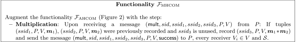
Fig. 3. Functionality \mathcal{F}_{\text{MHCOR}}
