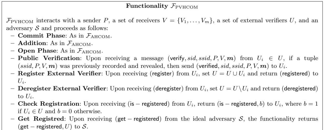
Fig. 14. Functionality \mathcal{F}_{\text{PVHCOM}}
