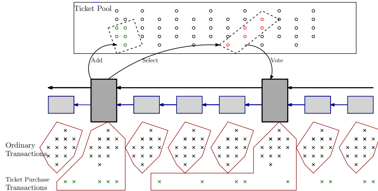
Fig. 1. The structure of Goshawk. The tickets are denoted by dots, the transactions are denoted by cross marks, the keyblocks are denoted by big rectangles, and the microblocks are denoted by small rectangles. A keyblock contains transactions and add tickets into ticket pool. Meanwhile, a keyblock pseudo-randomly selects tickets which will be removed from ticket pool. Chosen stakeholders vote for keyblock to validate it and votes will be contained by the next keyblock.
