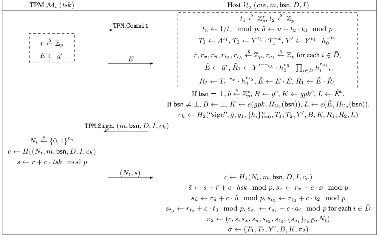
Fig. 2: The sign protocol of DAA OPT . For the case that bsn \neq \perp , B is set as \perp , as e(\bar{g}, H_{\mathbb{G}_2}(bsn)) can be computed offline by the verifier. The elements marked in the dashed box can be computed offline by the TPM and host. Again, TPM.Commit and TPM.Sign represent the TPM requests rather than real TPM 2.0 commands.
