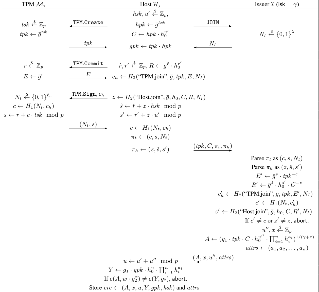
Fig. 1: The join protocol of DAA OPT . The notation TPM.Create, TPM.Commit and TPM.Sign represent the TPM requests of the following procedures: creating a TPM key , generating a commitment and generating a signature respectively. Note that they are not real TPM 2.0 commands.
