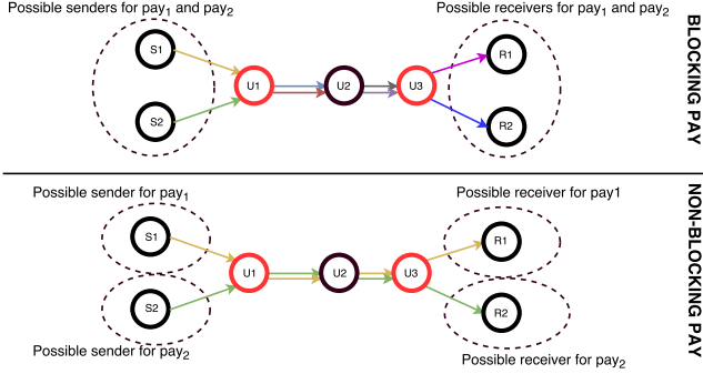
Figure 9: Illustrative example of tradeoff between concurrency and privacy. Each node represents a user: black nodes are honest and red are byzantine. In both cases, we assume two concurrent payments: S_1 pays R_1 and S_2 pays R_2 through the path U_1, U_2, U_3 . The color of the arrow denotes the payment identifier. Dashed ellipses denote the anonymity set for each case.
