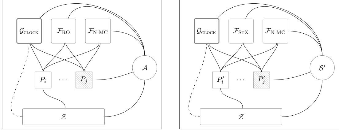
(a) In the real world parties have access to the global clock \mathcal{G}_{\text{CLOCK}} , the random oracle \mathcal{F}_{\text{RO}}^{\kappa} , and network \mathcal{F}_{\text{N-MC}} . Here, parties execute the Bitcoin protocol Ledger-Protocol
