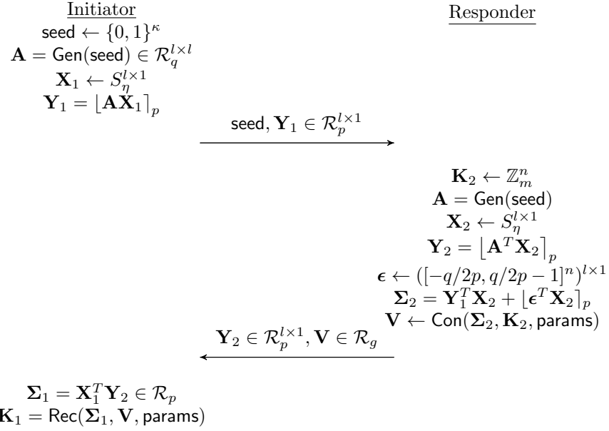
Figure 21: MLWR-based key exchange from AKC
