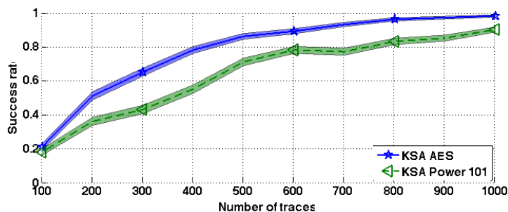
Fig. 6: Empirical success rate for S_{101} and S_{254} and \sigma^2 = 1 for (i)KSA.
