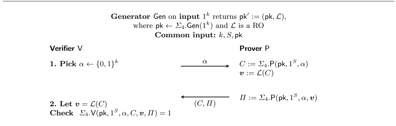
Fig. 4.1. The 2-messages (one-stage) PoSpace protocol \Sigma_2 = (\text{Gen}, \text{P}, \text{V}) .
