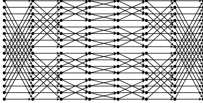
Fig. A.1. An example of 16-superconcentrator: the Butterfly Graph
