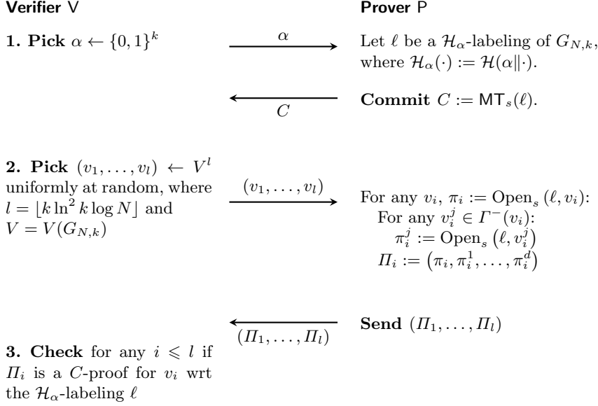
Fig. 3.1. The 4-message PoSpace protocol \Sigma_4 .
