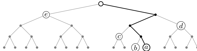
Fig. B.1. An example of opening: c = (a, b, c, d, e)
