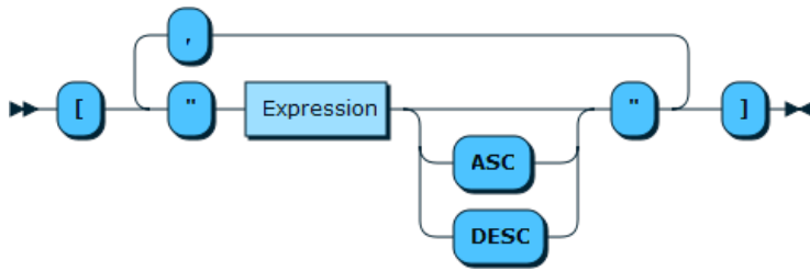
Figure 11.28 SortExprStrList
