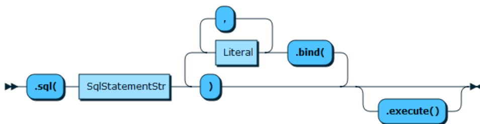
Figure 11.2 SqlExecute
