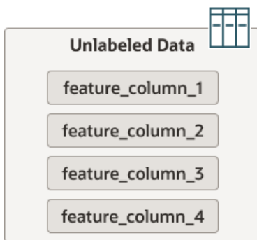
Figure 3.3 Unlabeled Data
