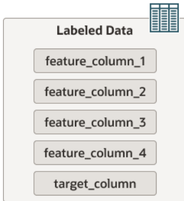
Figure 3.2 Labeled Data
