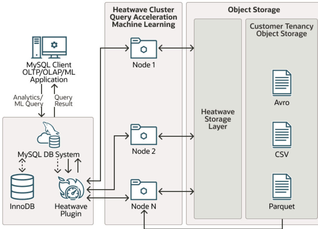
Figure 1.1 HeatWave Architecture
