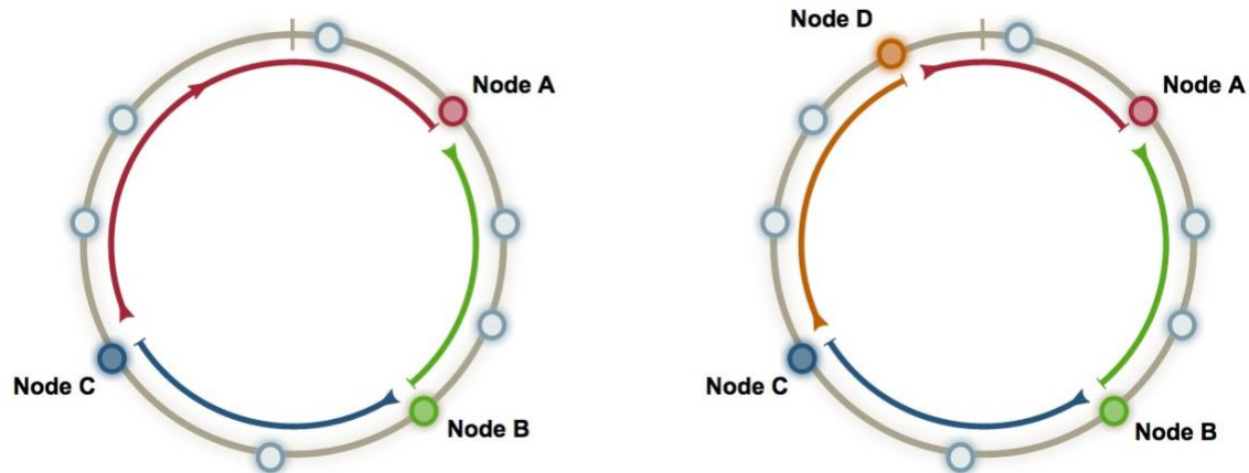
Consistent hashing
