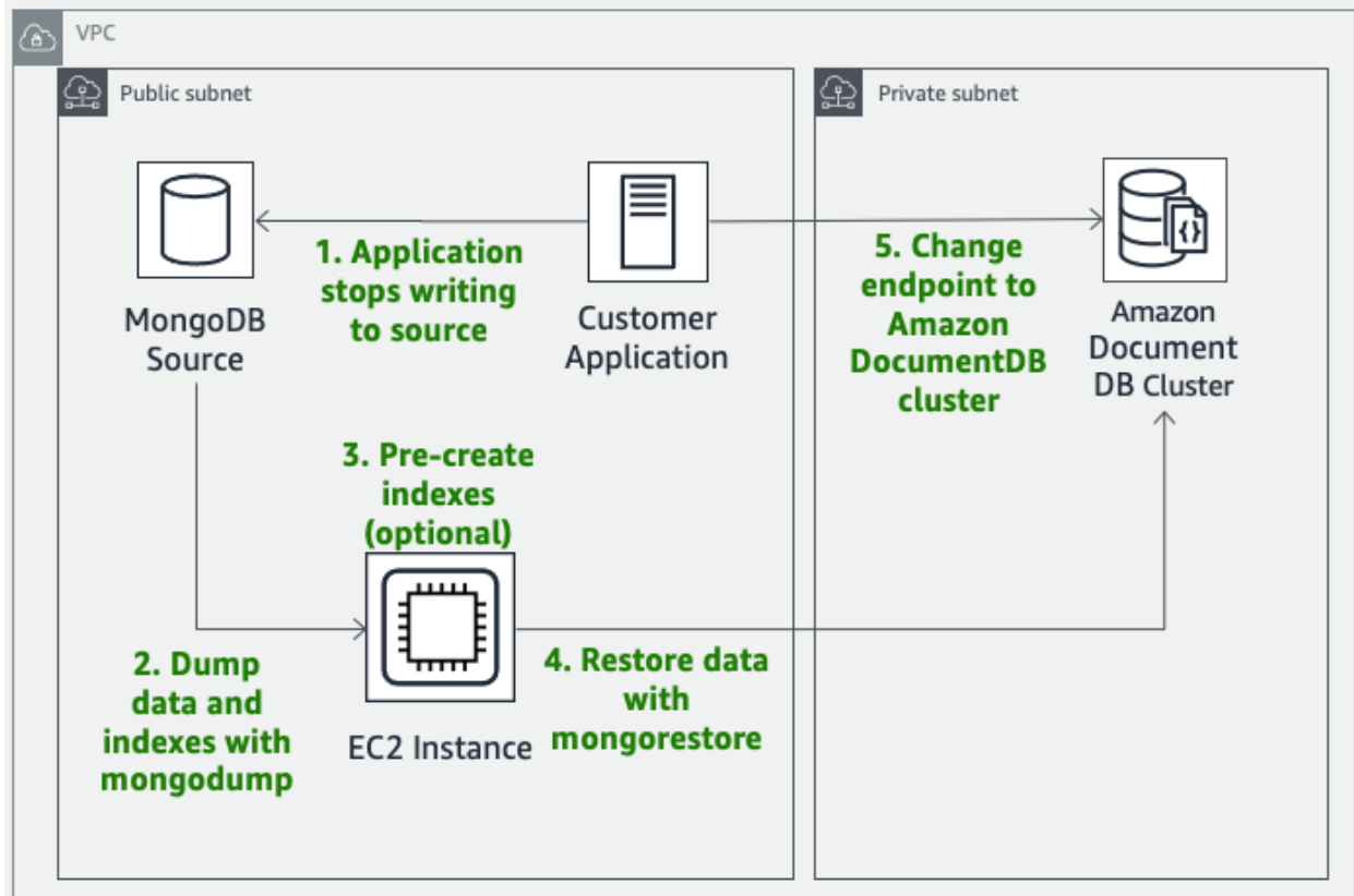
Figure 15: Offline migration approach
