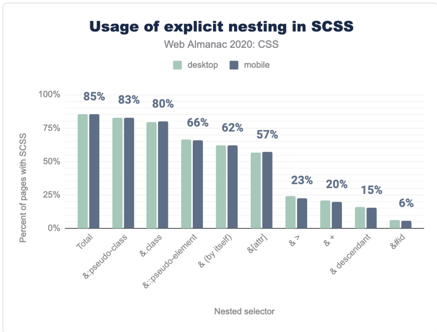
図1.73. usage-of-explicit-nesting-in-scss.
