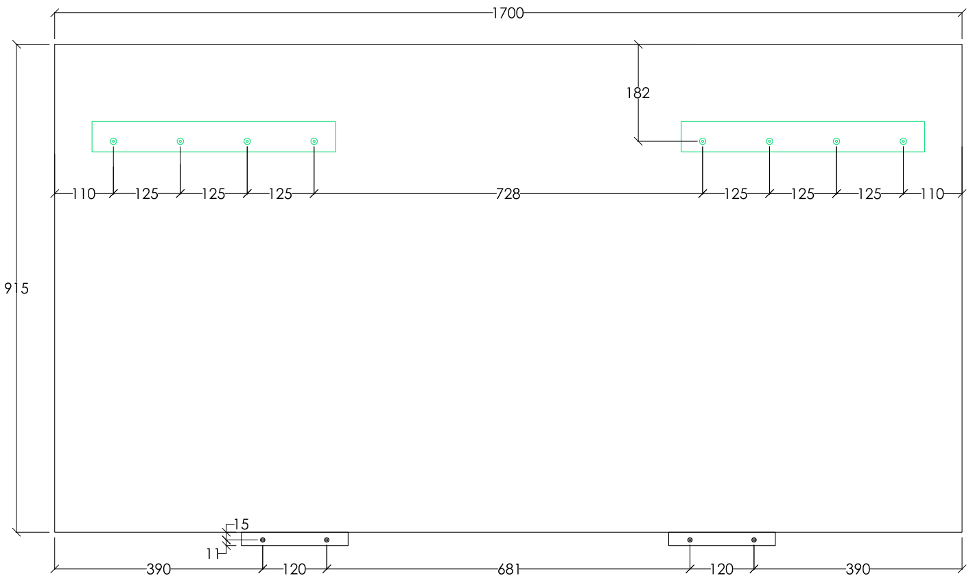
WALL MOUNTING HOLE DETAIL
