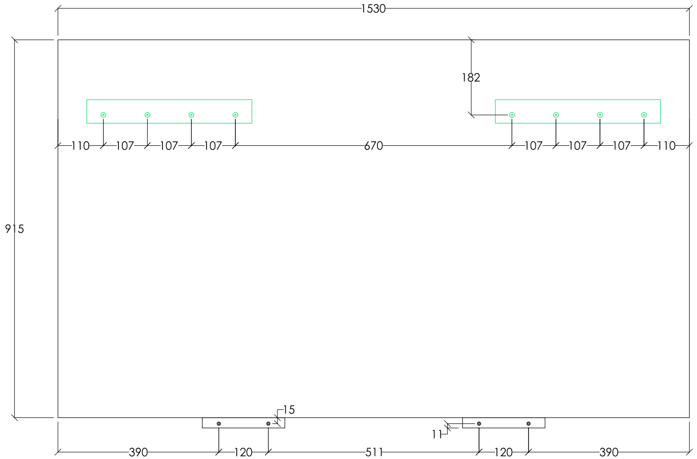
WALL MOUNTING HOLE DETAIL
