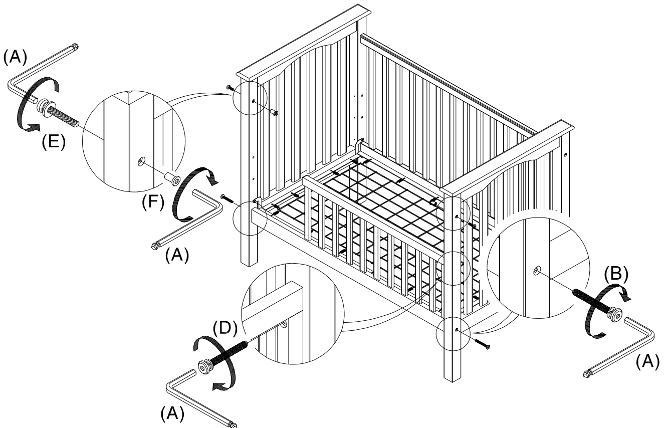
(B) Bolt 2x (from step 2) Boulons 2x (de l'étape 2)
