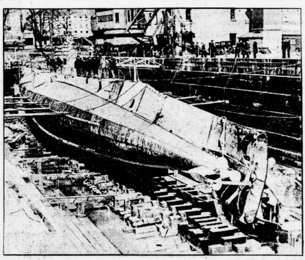
SUBMARINE IN DRY DOCK AFTER BEING AGROUND THREE MONTHS. The Navy's S-19, which ran aground at Orleans, Mass., was recently floated and towed to the Boston navy yard, where it is undergoing repairs. The rudder and propellers of the craft were badly damaged, and many of the plates were sprung.
