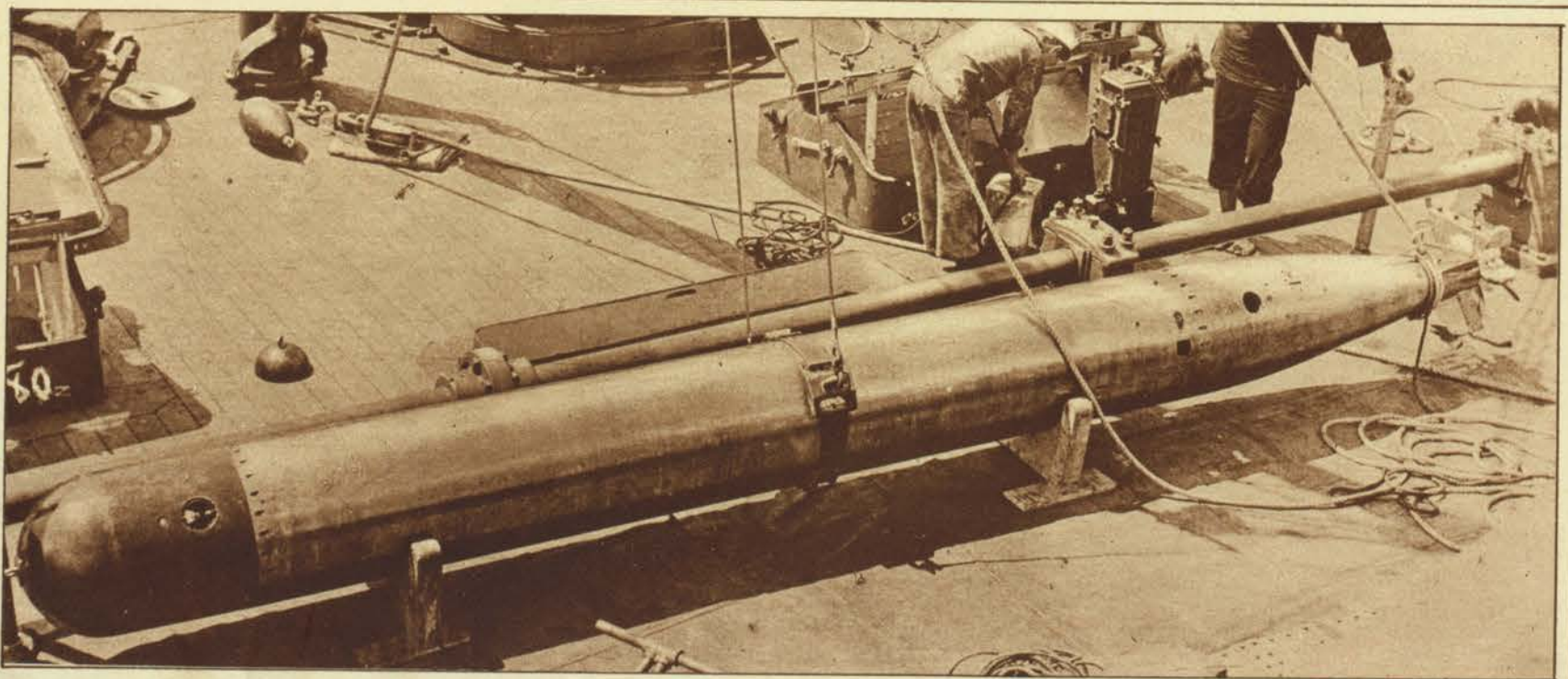
TORPEDO OF THE 21-INCH TYPE BEING GOTTEN READY TO BE LOWERED INTO THE HOLD OF THE OKLAHOMA. IT IS EXPELLED FROM THE TUBE BY COMPRESSED AIR, IS SELF PROPELLING, EXPLODES ON CONTACT, AND HAS A CHARGE OF 200 POUNDS OF GUN COTTON.
