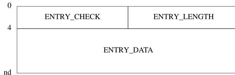
Figure 3-2. Entry Point Code Block
