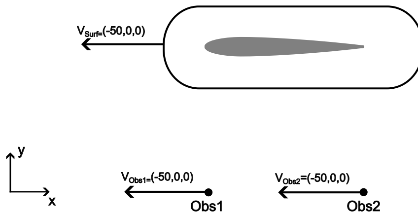
Fig. 4: FWH simulation of an airfoil, with quiescent medium co-ordinate transformation applied
