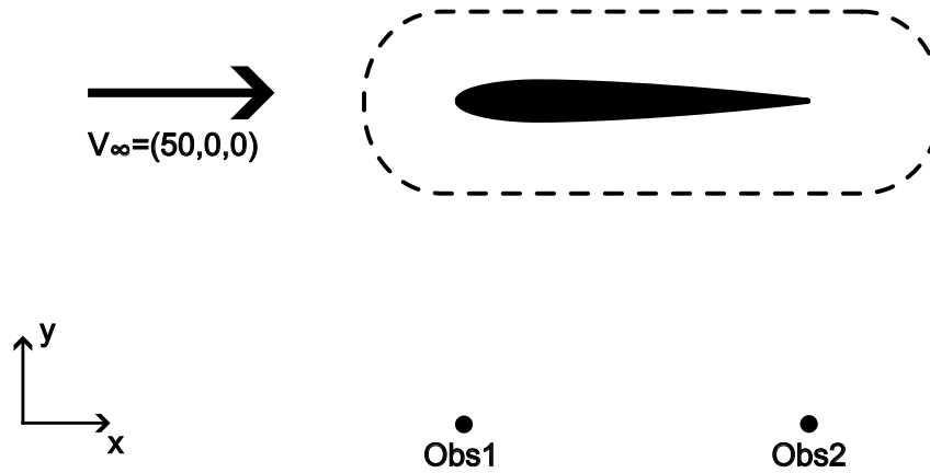
Fig. 3: CFD simulation of an airfoil, including an FWH surface
